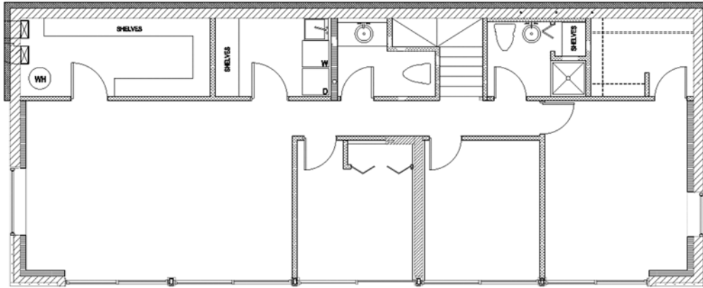
WALK-OUT BASEMENT PLAN
