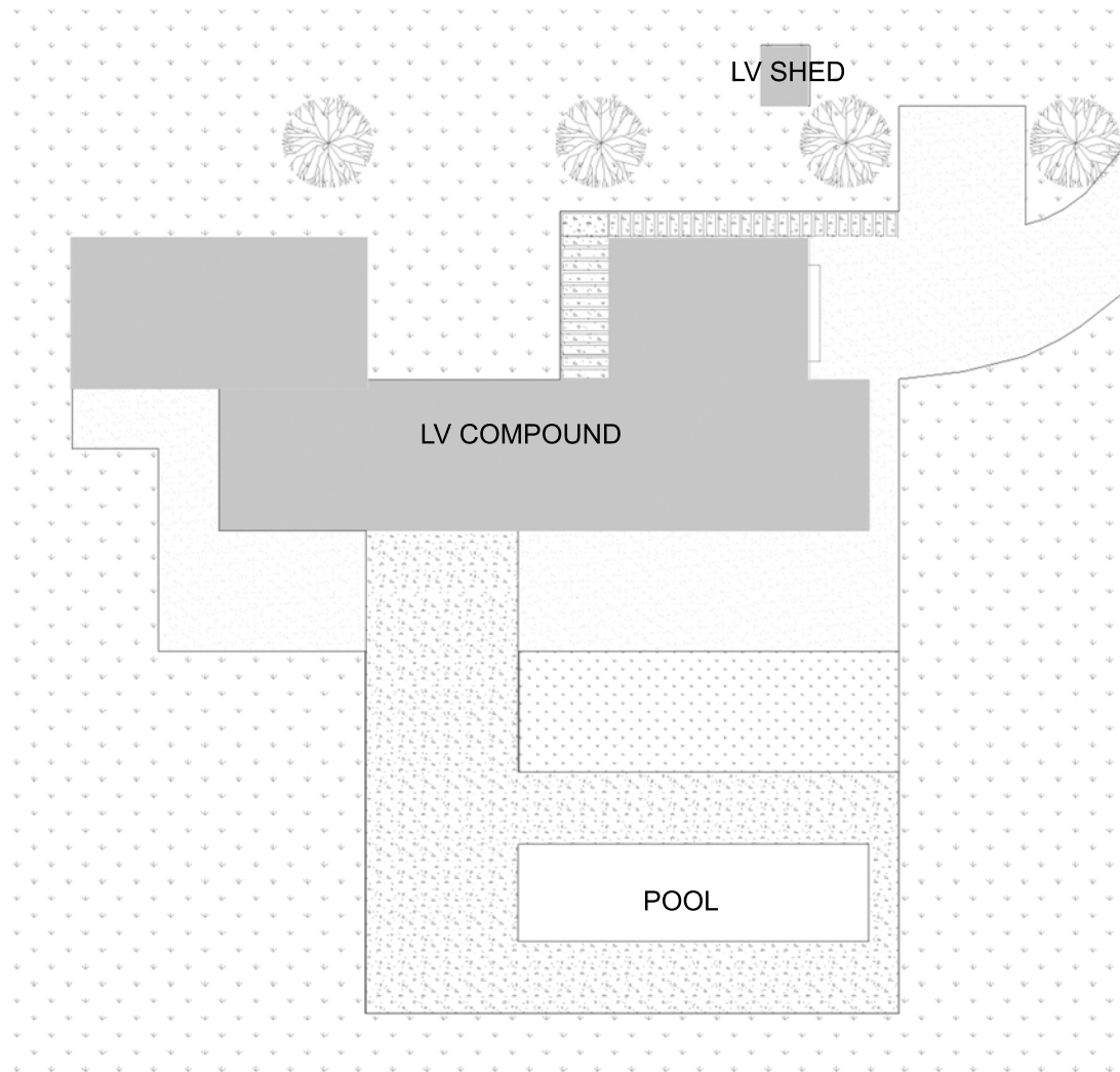
SITE PLAN
