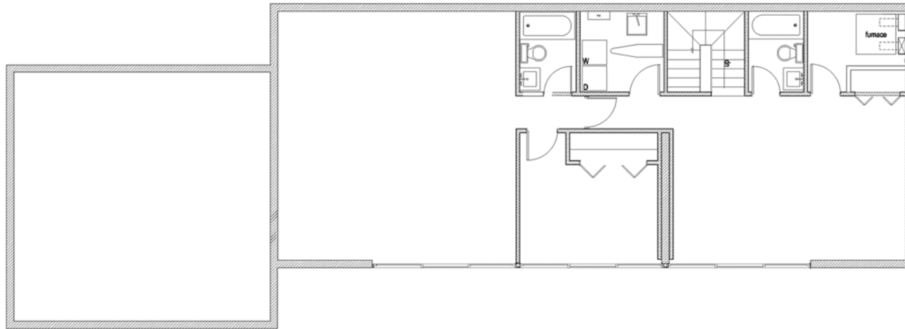
BASEMENT PLAN
